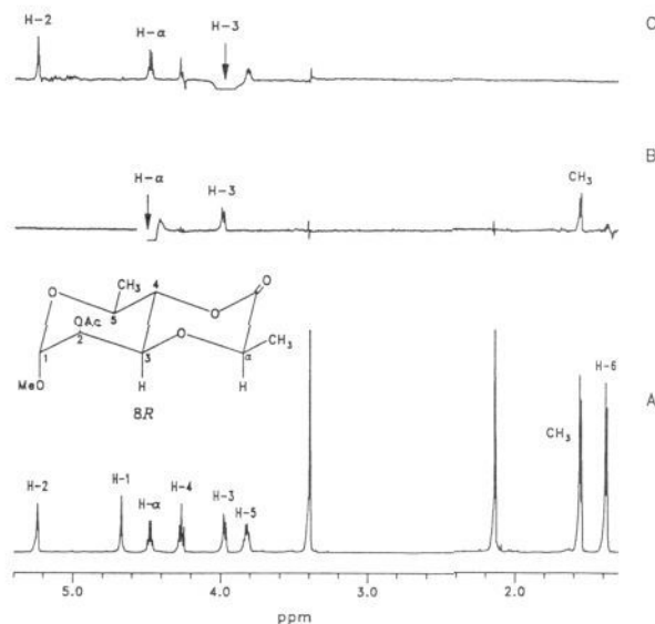
Figure 2. 1 H NMR spectrum of the acetylated lactone derivative of methyl 3- O -[( R )-1-carboxyethyl]- \alpha -L-rhamnopyranoside ( 8R ) (A), NOE difference spectra obtained by irradiation of the lactyl \alpha -proton resonance (B), and the H-3 resonance (C).
