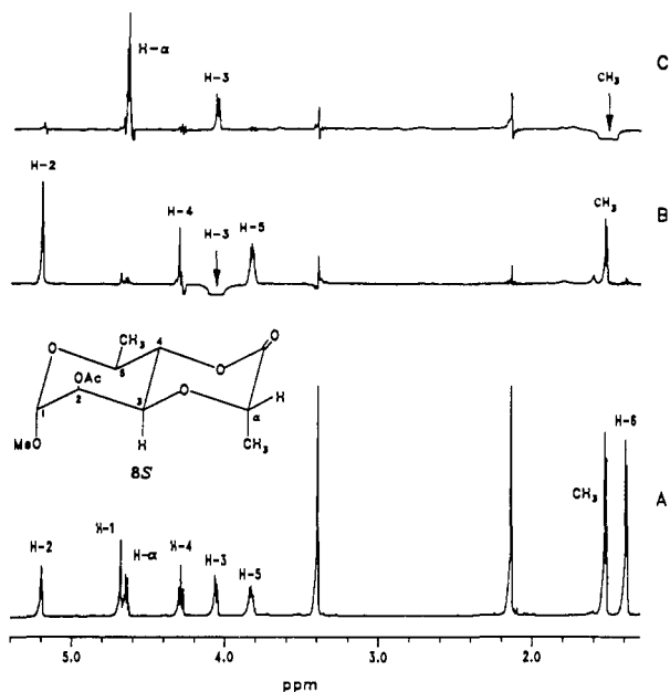
Figure 3. 1 H NMR spectrum of the acetylated lactone derivative of methyl 3- O -[( S )-1-carboxyethyl]- \alpha -L-rhamnopyranoside (8S) (A), NOE difference spectra obtained by irradiation of the H-3 resonance (B), and the lactyl methyl proton resonance (C).
