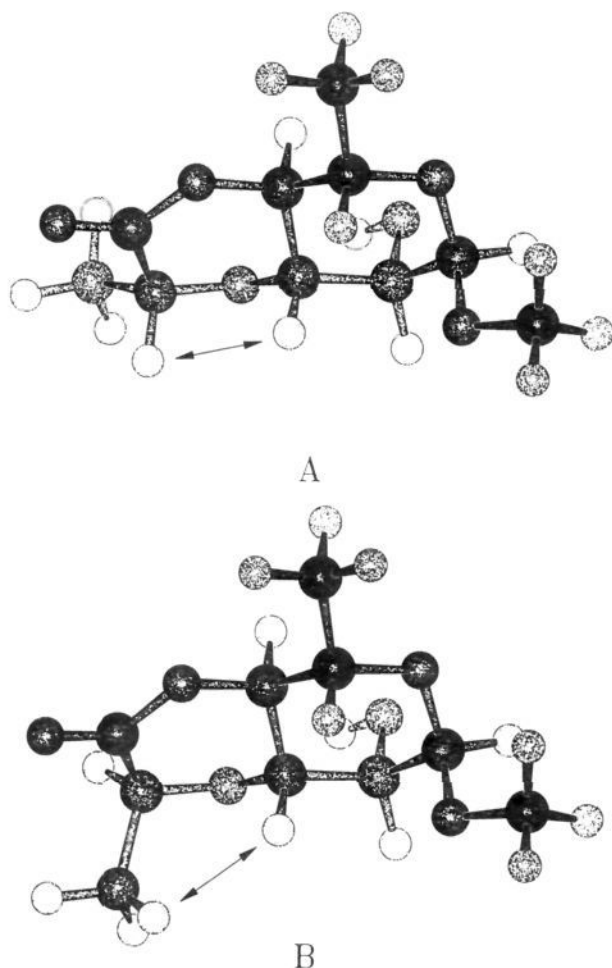
Figure 1. Computer generated models for the (A) ( R )- and (B) ( S )-3,4-lactone derivatives of methyl 3- O -(1-carboxyethyl)- \alpha -L-rhamnopyranoside.
