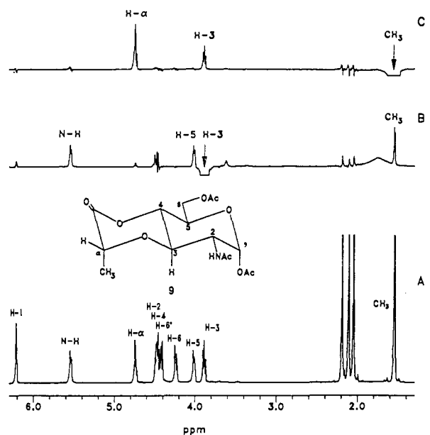
Figure 4. 1 H NMR spectrum of the acetylated lactone derivative of 2-amino-2-deoxy-3- O -[( R )-1-carboxyethyl]- \alpha -D-glucose (9) (A), NOE difference spectra obtained by irradiation of the H-3 resonance (B), and the lactyl methyl proton resonance (C).
